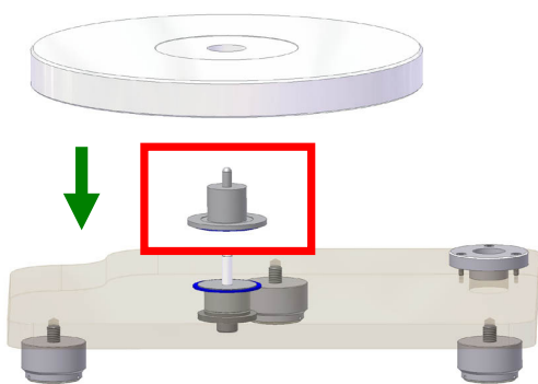
Pic. 3: Placing the bearing
