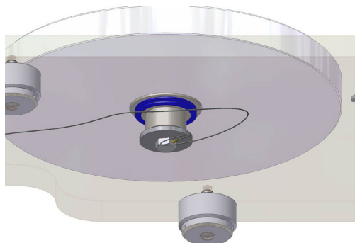
Pic. 14: Connecting the ground wire to the turntable
