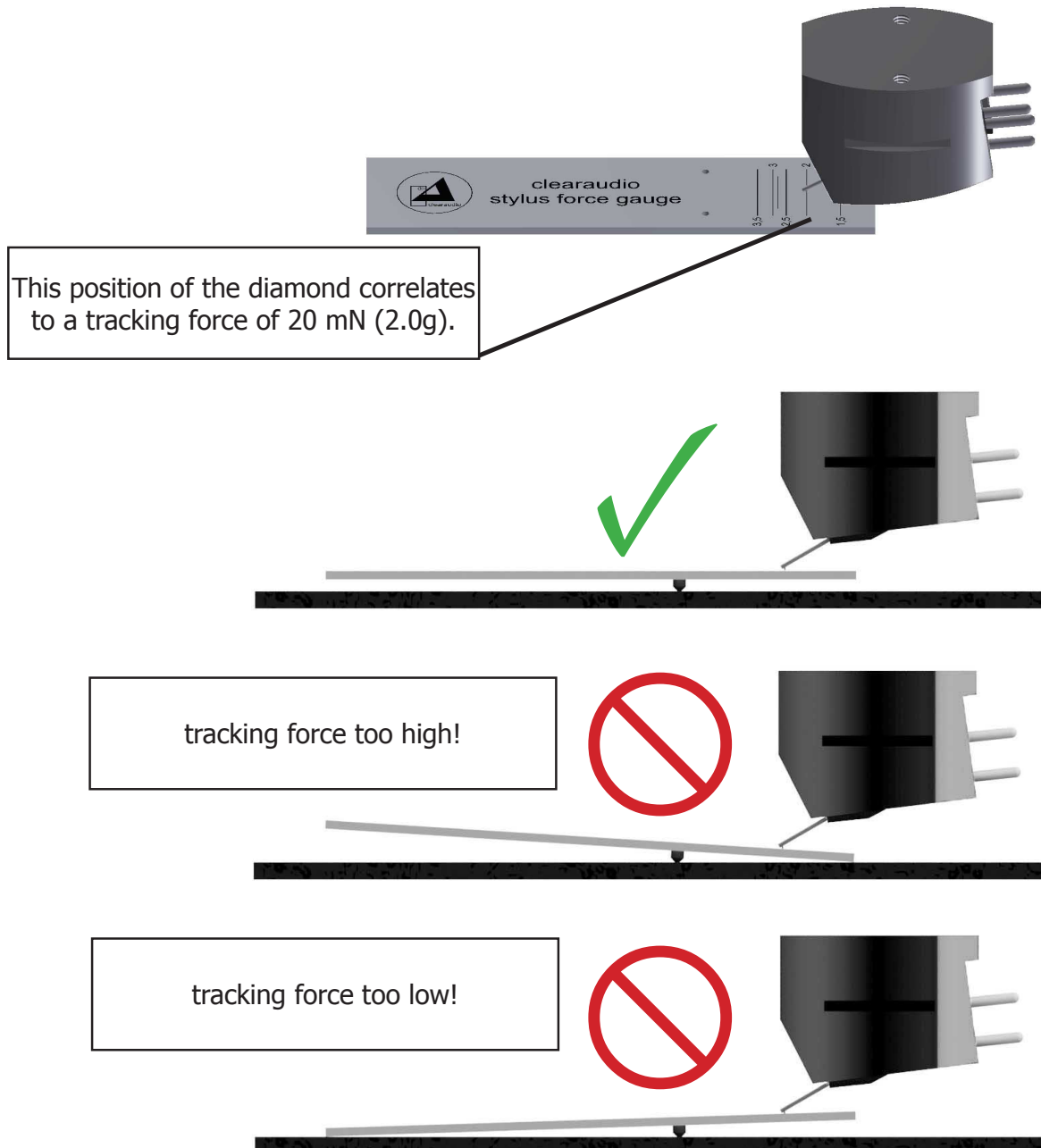
Pic. 8: Use of the Smart Stylus Gauge
