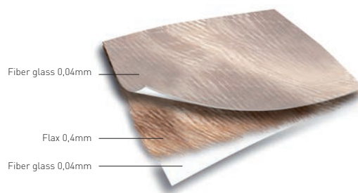
> Flax sandwich Details for midrange driver
