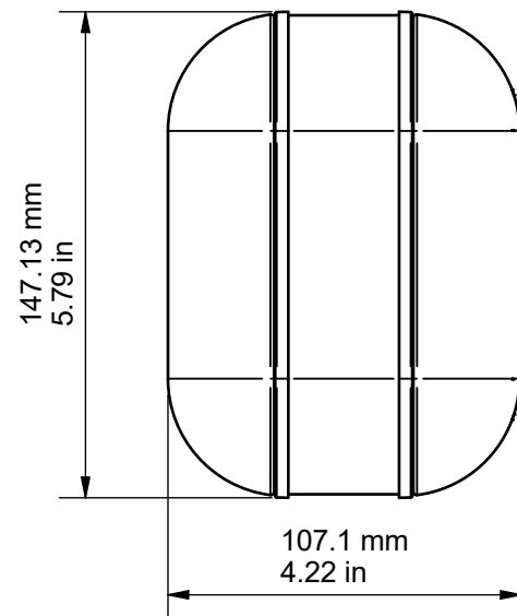
SIDE (LEFT)
