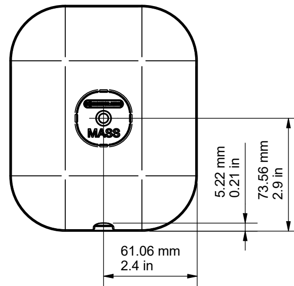
REAR
