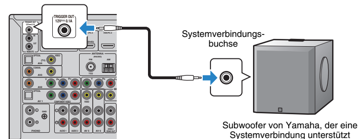
Buchse TRIGGER OUT
